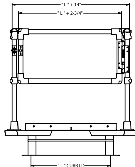
ROOF HATCH & SAFETY RAILS FRONT VIEW (ROOF HATCH COVER REMOVED FOR A BETTER VIEW OF THE RAIL SYSTEM)
